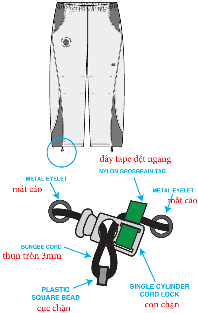
INTERIOR BUNGEE CORD CONSTRUCTION DETAILS-1
