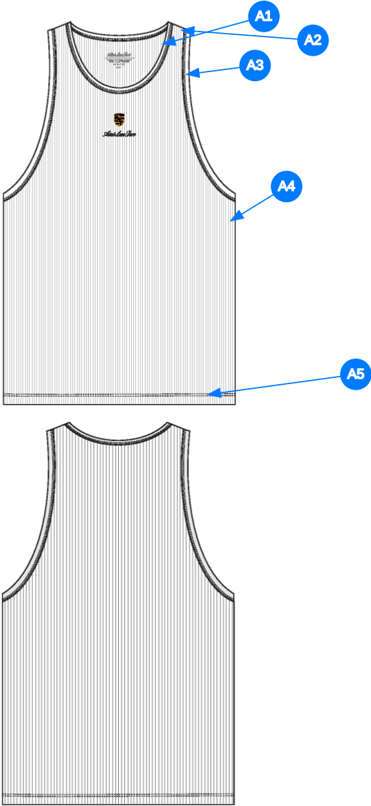
4_STITCHING DETAILS-1
