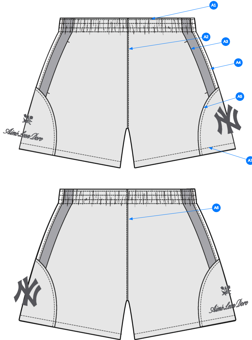
4_STITCHING DETAILS_12-1
