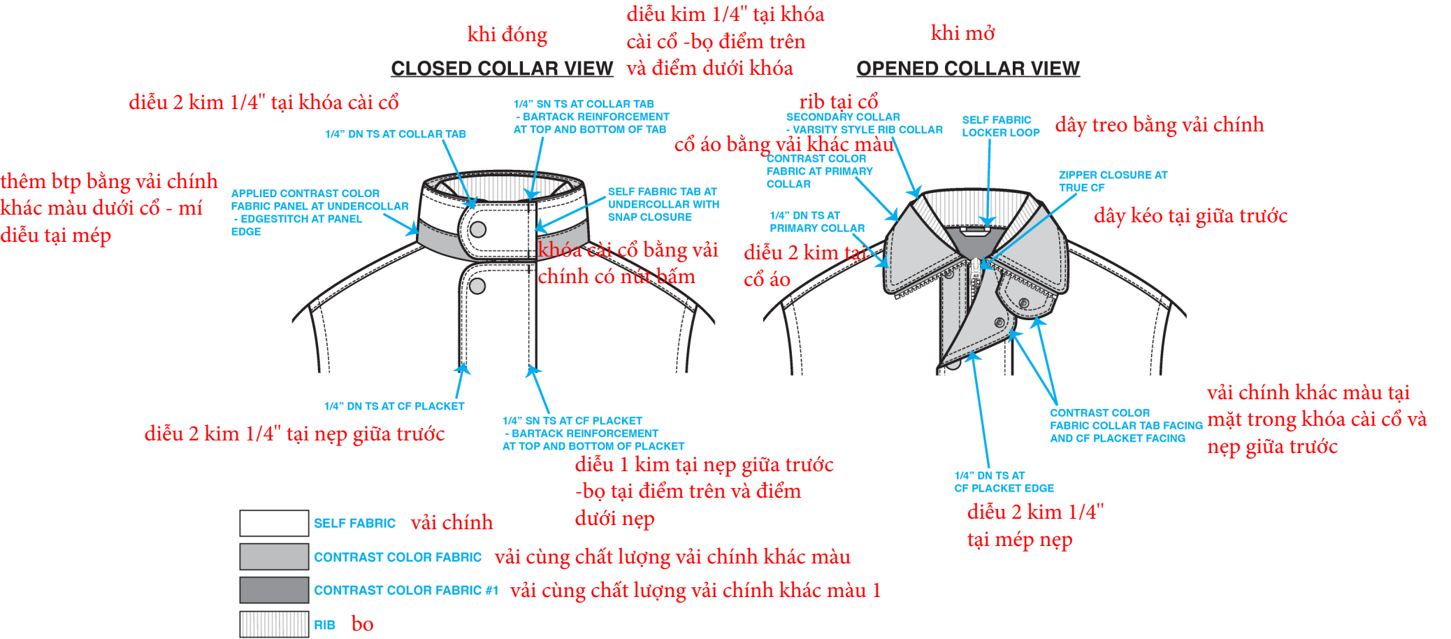
06_COLLAR DETAIL VIEW
