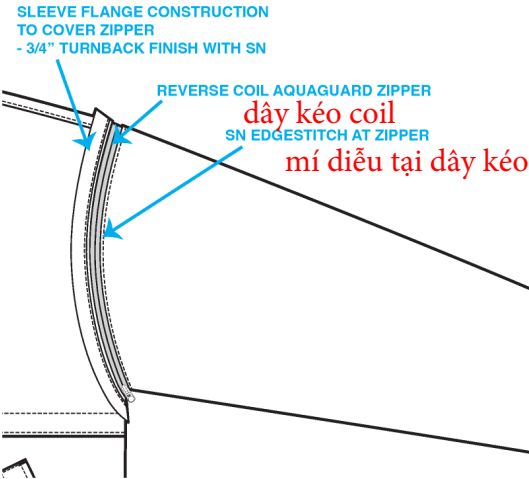
khi đóng ATTACHED SLEEVE VIEW
