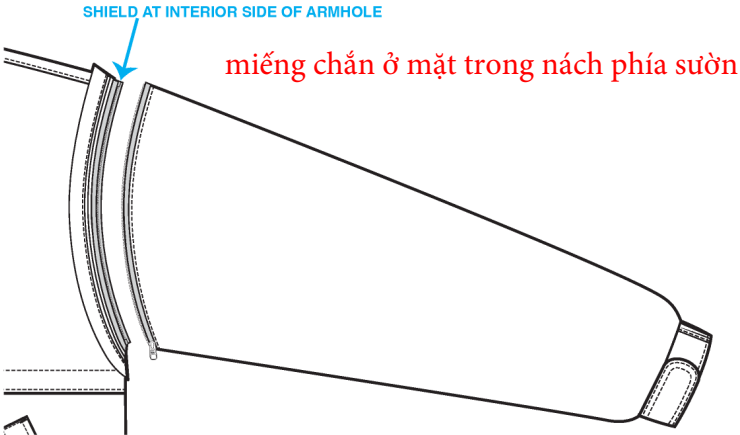
khi mở DETACHED SLEEVE VIEW
