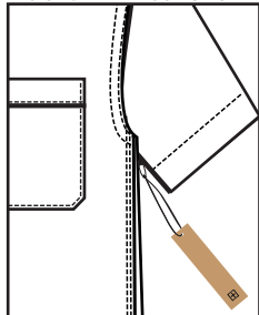
KS-002 - ATTACH SWING TAG TO LHS UNDER ARM JUNCTION
