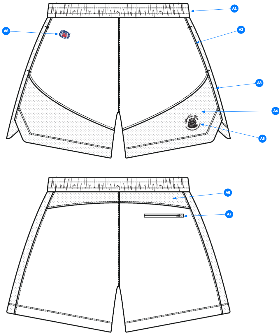
3_CONSTRUCTION DETAILS-1
