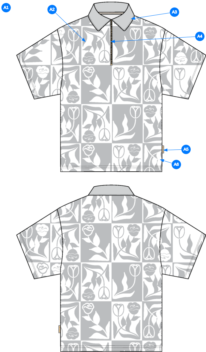
3_Construction Details-1
