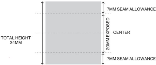
FLAG LABEL UNFOLDED DIMENSIONS:
