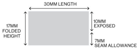
FLAG LABEL FOLDED DIMENSIONS:
